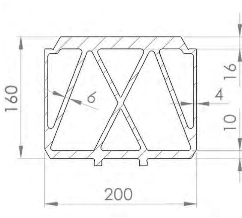
> Figure 5-24 Joiner profile between top deck and bulkhead, dimensions
