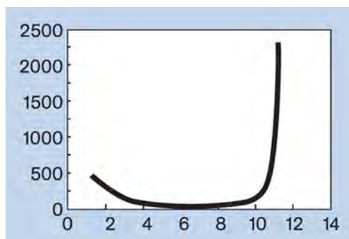
> Figure 3-17 Corrosion rate vs. pH
