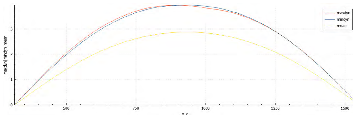
> Figure 6-4 Plate concept: Lateral displacement [m] of the bridge girder.
