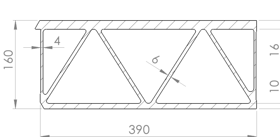
> Figure 5-21 Top deck panel toward joiner profile in bulkhead (right side)
