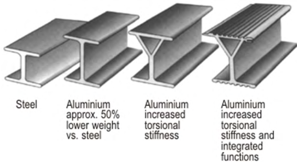
> Figure 3-16 Design of aluminium extrusion (AZOM)
