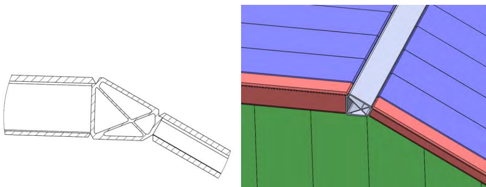
> Figure 5-30 Possible joiner profile 2
