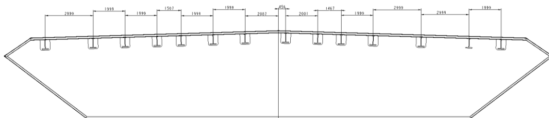
> Figure 5-4 Distribution of lateral spacing between longitudinal beams
