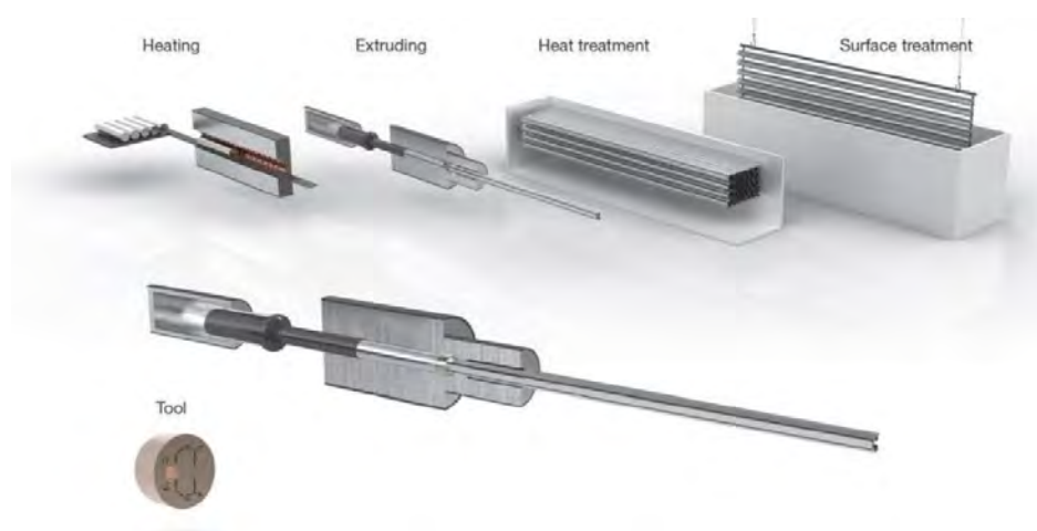
> Figure 3-8 Aluminium extrusion process (Hydro)
