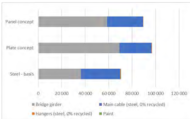
> Figure 9-6 CO 2 footprint based on Hydro European average material [ton CO 2 ]
