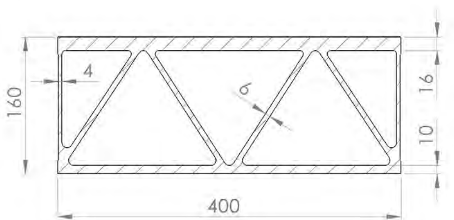
> Figure 5-20 Top deck panel
