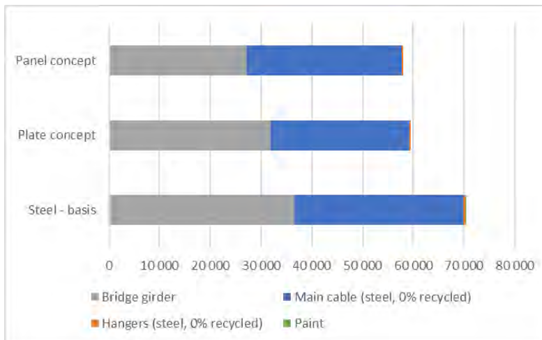
> Figure 9-4 CO 2 footprint based on Hydro 75R [ton CO 2 ]
