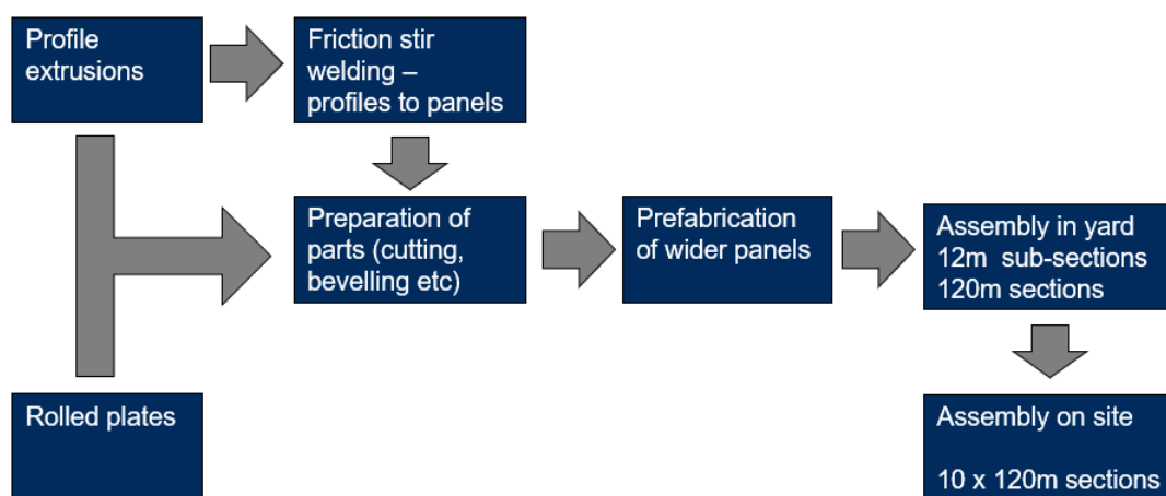
> Figure 8-1 Assembly flowchart
