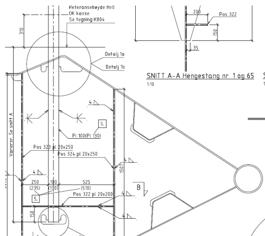
> Figure 5-16 Hanger joint from Hardangerbrua
