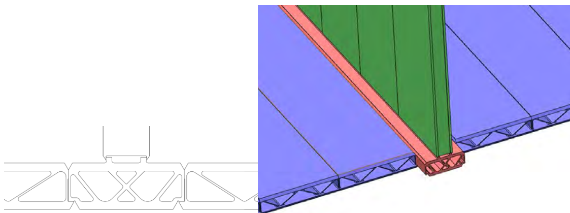
> Figure 5-27 Joiner profile between bottom deck and transverse bulkhead
