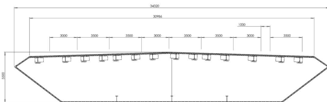
> Figure 5-1 Panel concept, cross-section
