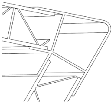
> Figure 5-8 Joining upper side panel to lower side panel using joiner profile
