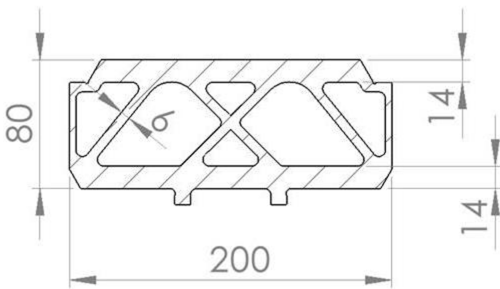
> Figure 5-26 Joiner profile between bottom deck and transverse bulkhead, dimensions
