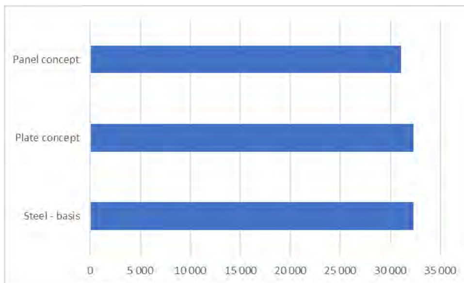
> Figure 9-9 Net CO 2 footprint including avoided burden [ton CO 2 ]
