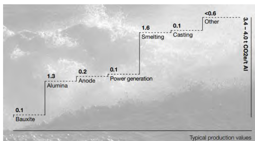
> Figure 9-3 Hydro 4.0 carbon footprint
