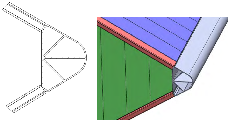
> Figure 5-31 Possible joiner profile 3
