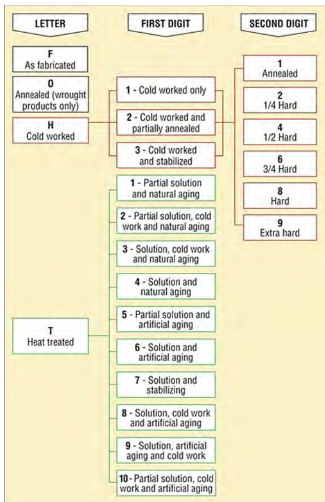
> Figure 3-5 Aluminium temper designation
