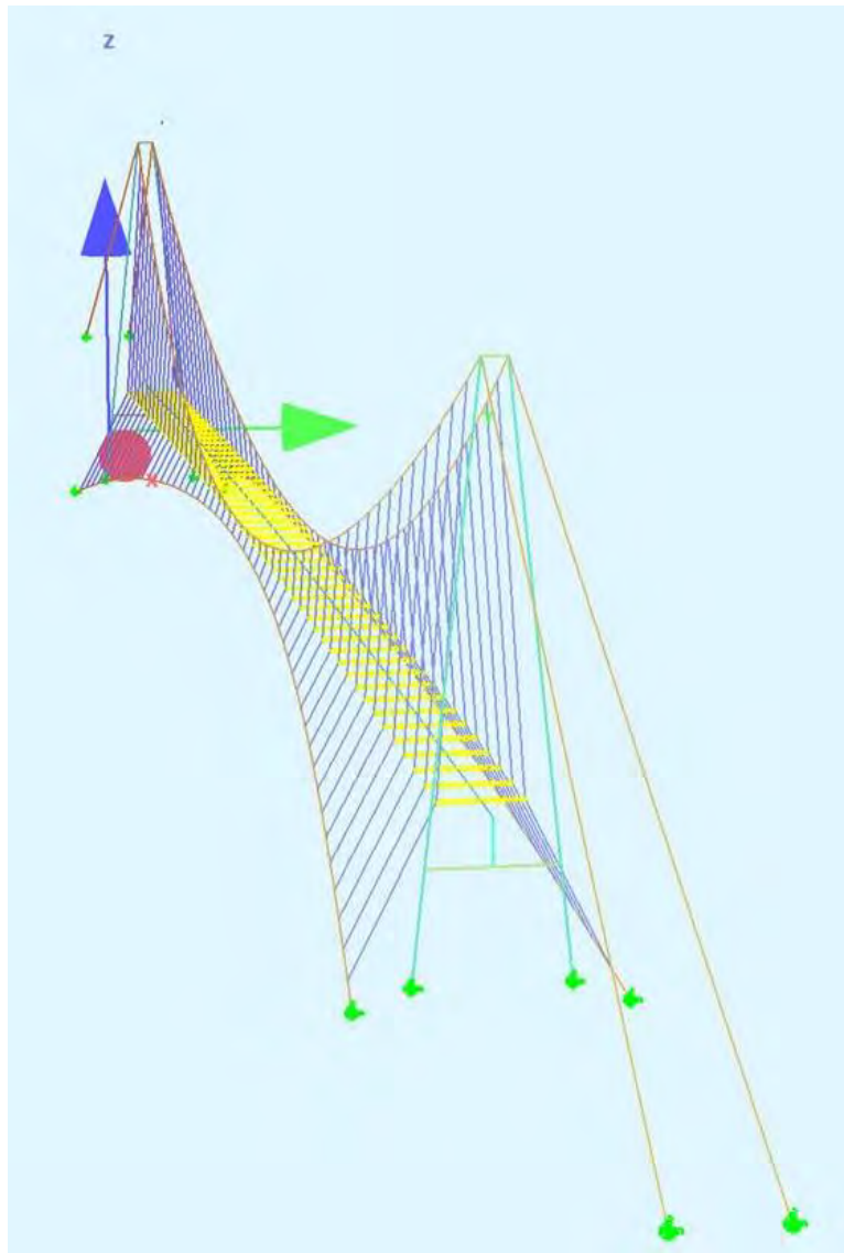
> Figure 5-34 Example of partly horizontal, partly vertical inverted cable suspension bridge model.
