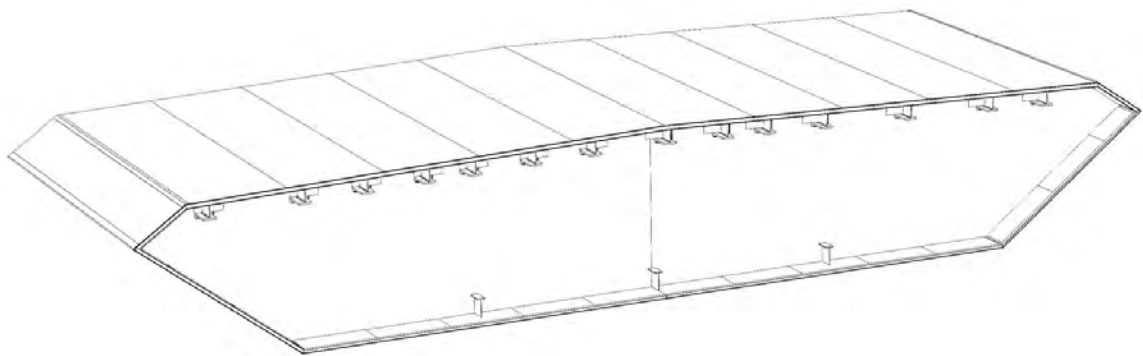
> Figure 5-11 Main view of a girder section with bulkhead
