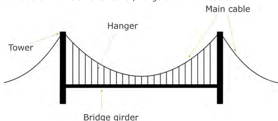
> Figure 1-1 Suspension bridge elements included in the cost figures
