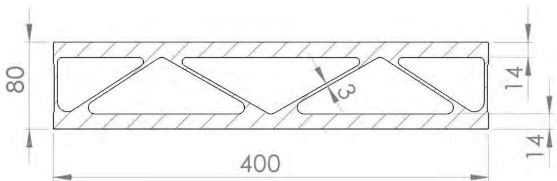
> Figure 5-22 Bottom and side deck panel
