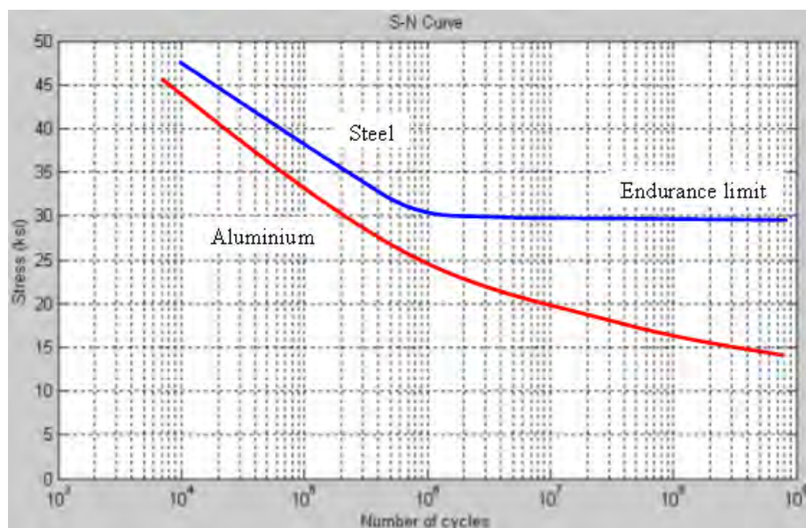
> Figure 3-15 Representative SN-curves for steel and aluminium
