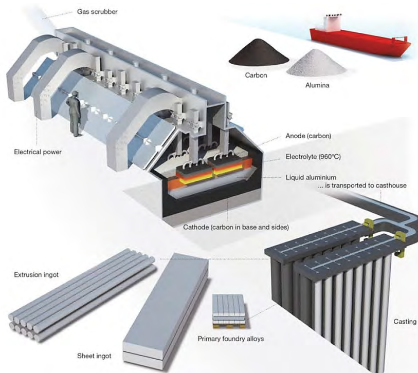
> Figure 3-6 Aluminium smelting process (Hydro)
