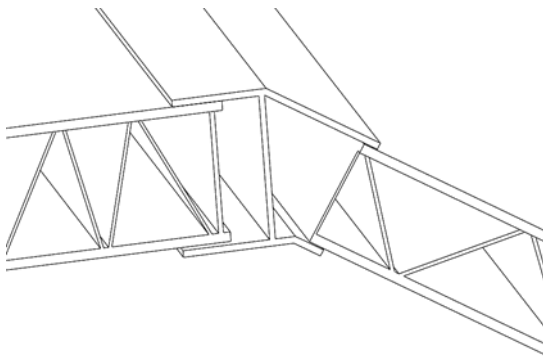
> Figure 5-9 Joining lower side panel to bottom panel using joiner profile
