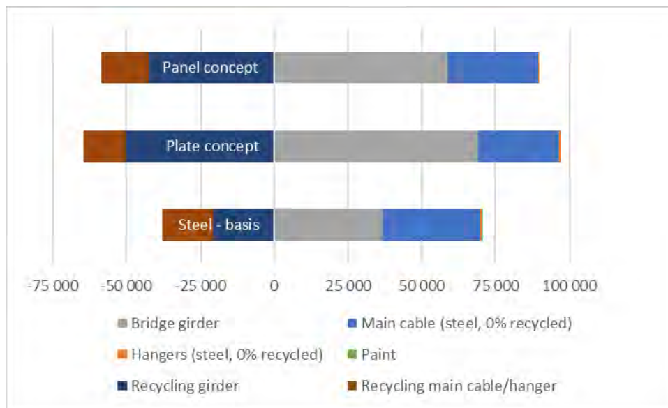
> Figure 9-8 CO 2 footprint including avoided burden [ton CO 2 ]
