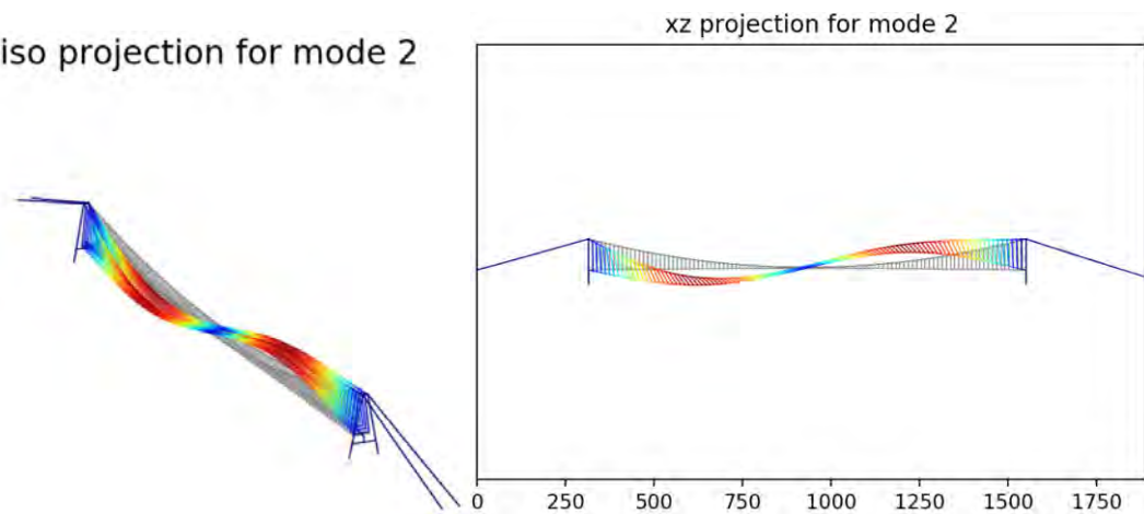
> Figure 6-6 The mode shape of the second eigenmode for the plate concept
