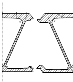
> Figure 5-2 Example of weld preparations that are integrated in the profiles
