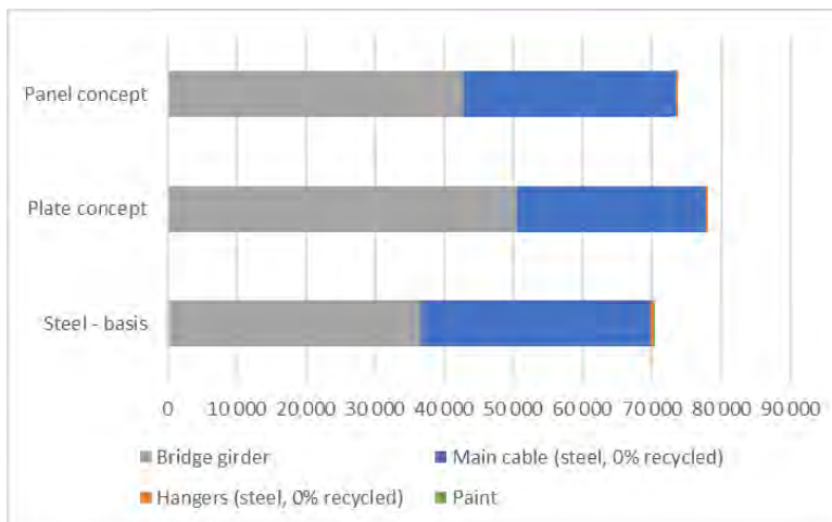
> Figure 9-5 CO 2 footprint based on Hydro 4.0 material [ton CO 2 ]
