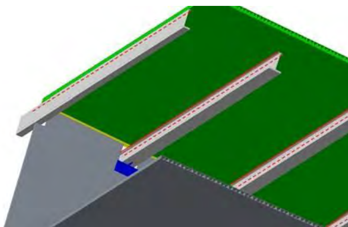
> Figure 7-1 The weld joining the deck beams and top deck panel (W2 - 7mm fillet)
