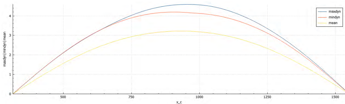
> Figure 6-3 Panel concept: Lateral displacement [m] of the bridge girder
