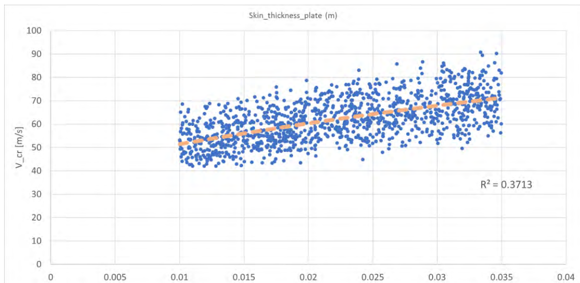
> Figure 4-6 Critical wind speed with respect to the skin thickness of the top and bottom plate
