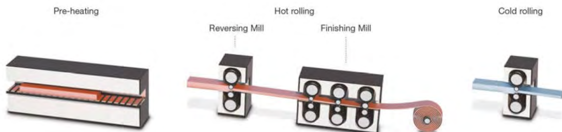
> Figure 3-7 Aluminium rolling process (Hydro)
