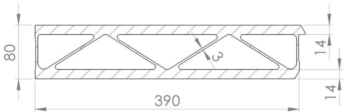
> Figure 5-23 Bottom and side deck panel towards joiner profile in bulkhead (right side)
