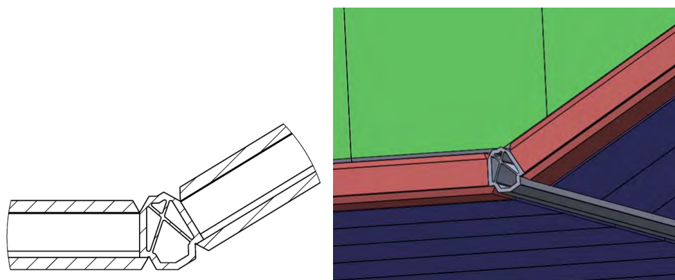
> Figure 5-32 Possible joiner profile 4
