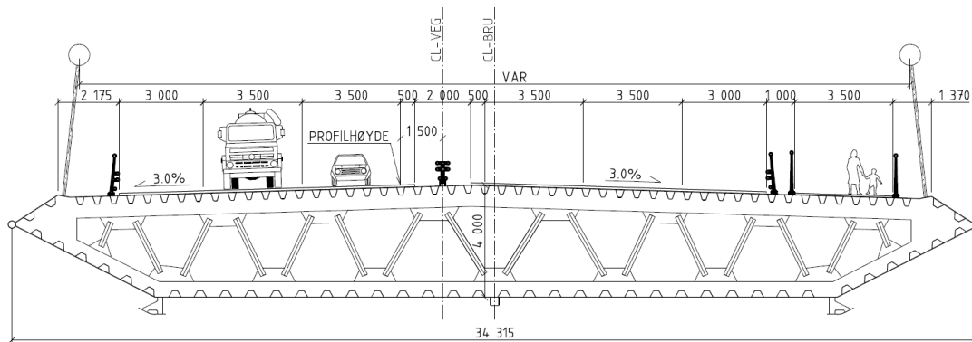
> Figure 5-35 Steel concept developed by Norconsult [11]
