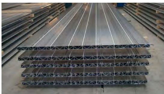
> Figure 3-14 Double welded FSW panels from hollow profiles
