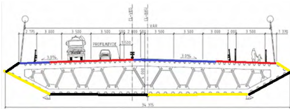
> Figure 5-28 Panel layout in the transverse bridge direction
