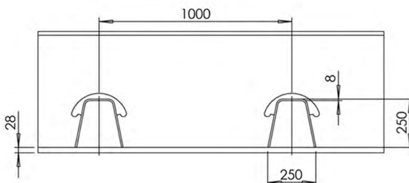
> Figure 5-13 Detail bottom plate skin
