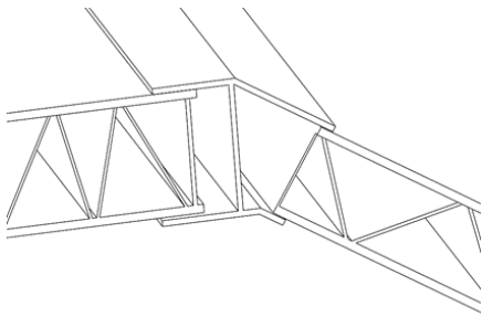
> Figure 5-7 Joining deck panel to upper side panel using joiner profile
