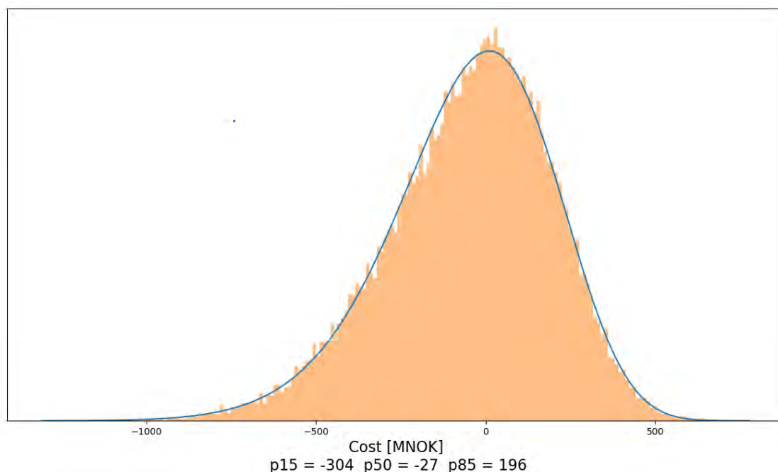
> Figure 6-7 Probability density with regards to difference in cost between the steel concept and the plated aluminium concept.
