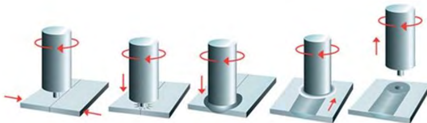
> Figure 3-12 Friction stir welding process (Hydro)
