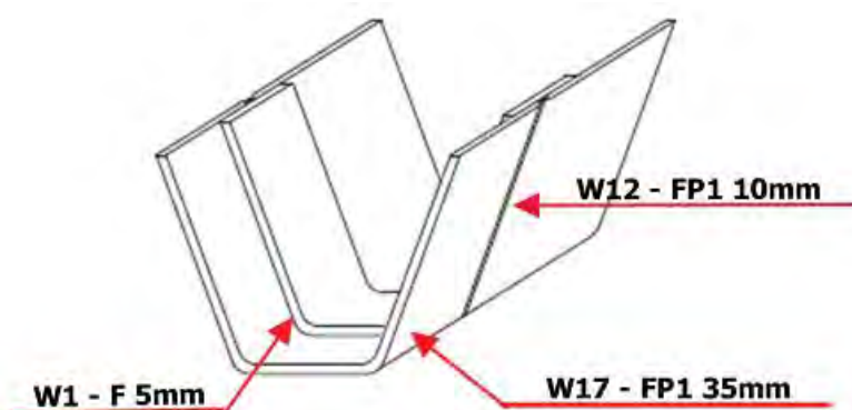
> Figure 7-2 Joining of stiffeners
