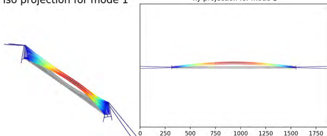
> Figure 6-5 The mode shape of the first eigenmode for the plate concept
