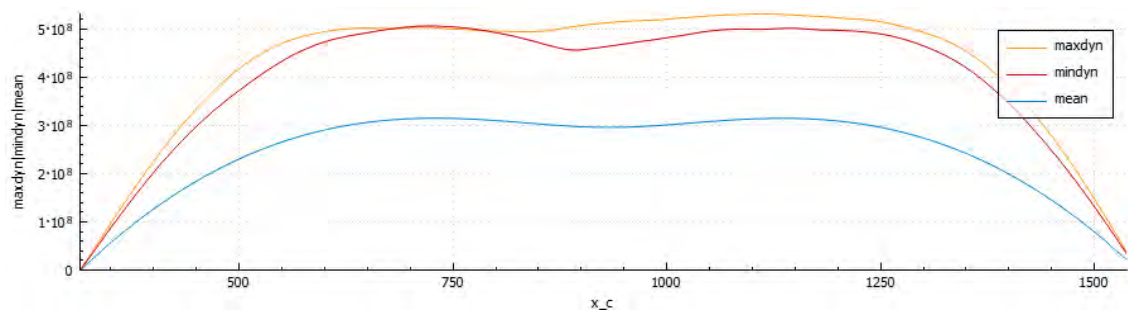
> Figure 6-1 Panel concept: Moment [Nm] about vertical axis. Maximum and minimum dynamic contribution and mean (static) contribution.
