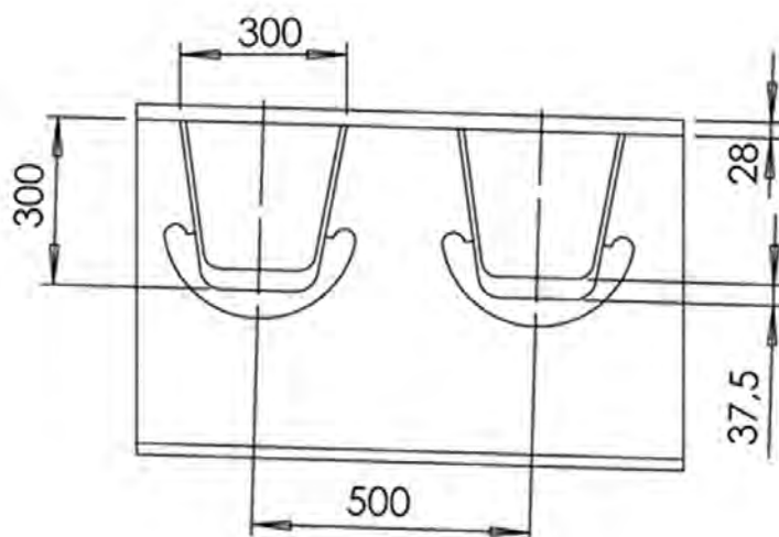
> Figure 5-14 Detail road deck
