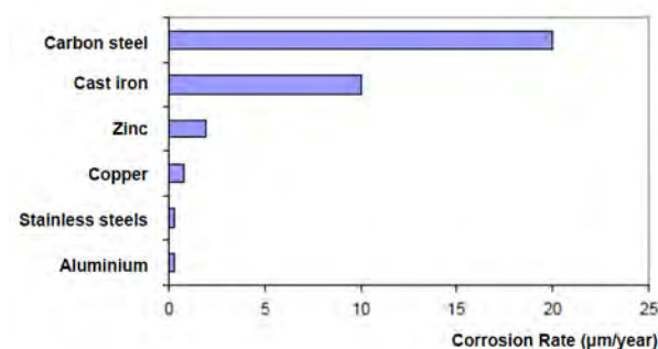
> Figure 3-18 Uniform corrosion in marine atmosphere
