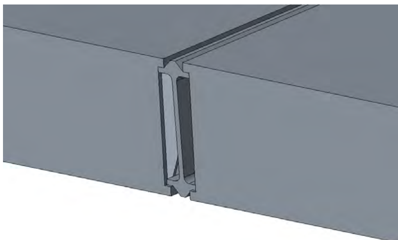
> Figure 5-5 Weld support profile for transversal weld of deck panels
