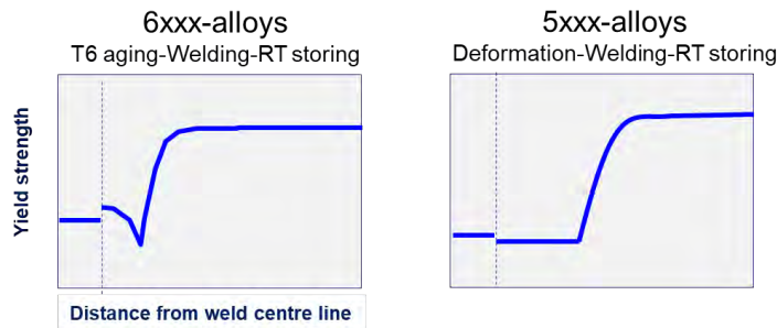
> Figure 3-11 Yield strength profile in welded joint (Hydro)
