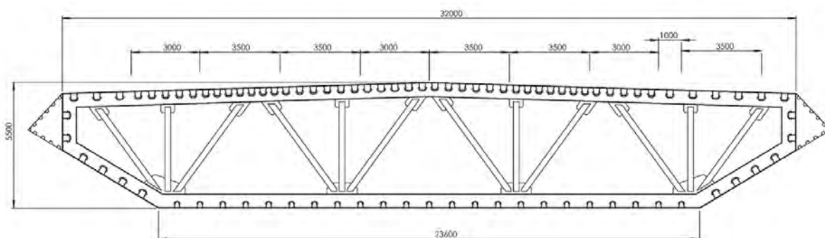
> Figure 5-15 Cross-section 2D
