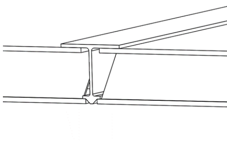
> Figure 5-6 Weld support profile or transversal weld of side/bottom panels
