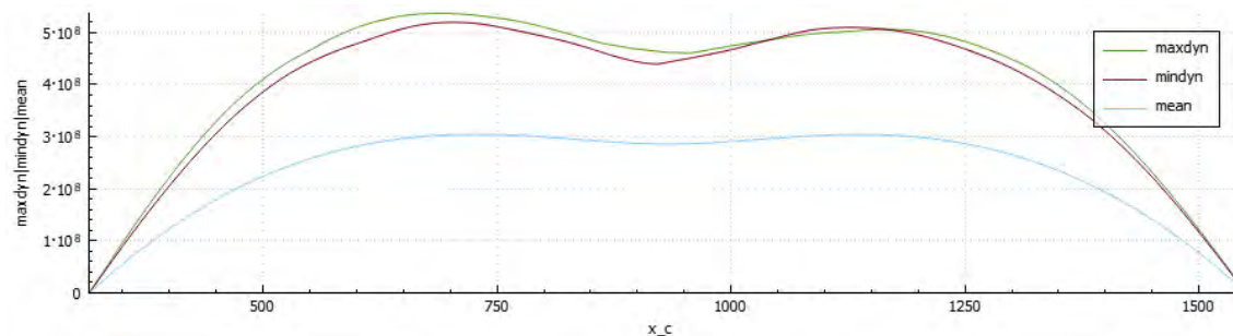
> Figure 6-2 Plate concept: Moment [Nm] about vertical axis. Maximum and minimum dynamic contribution and mean (static) contribution.
