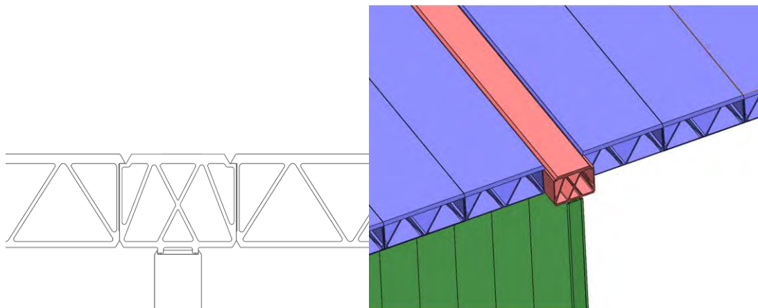
> Figure 5-25 Joiner profile between top deck and bulkhead
